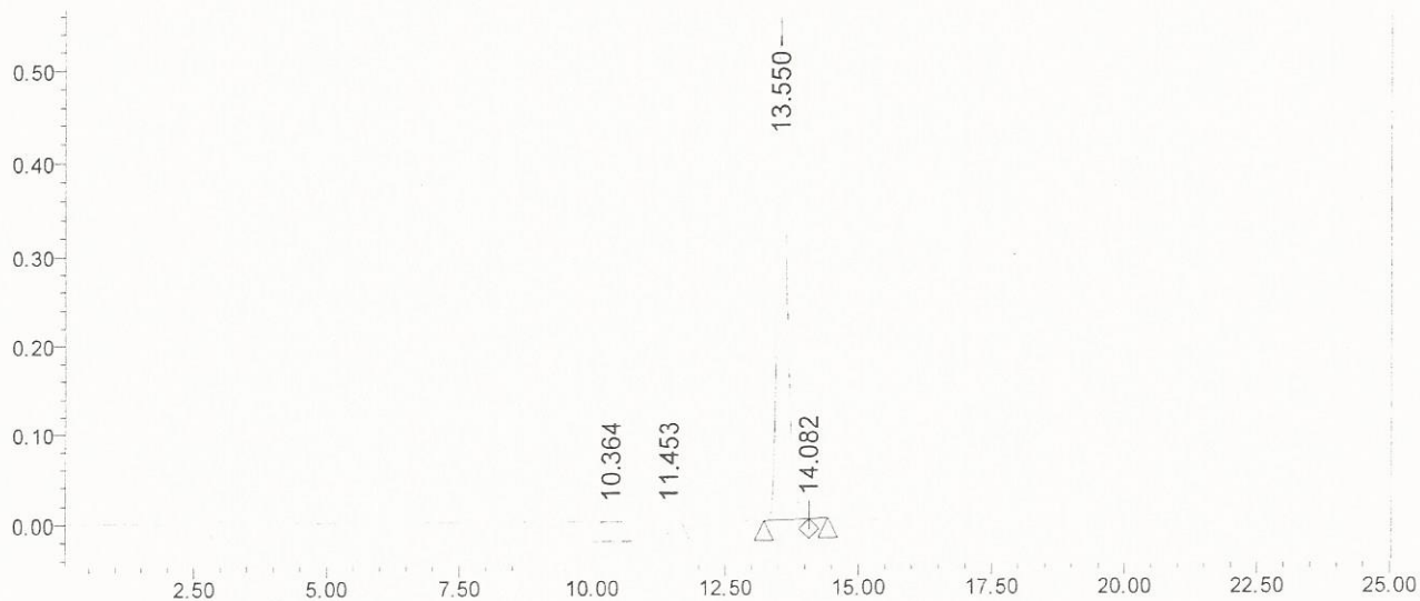
Auto-Scaled Chromatogram
